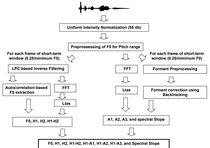
Figure 1: Diagram of feature extraction algorithm
